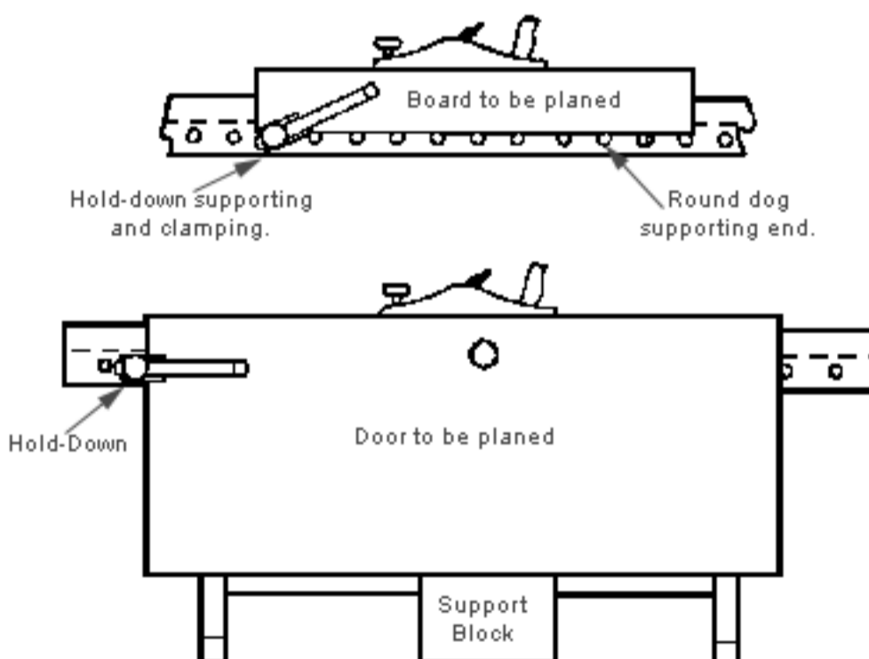
Fig. 2: Typical uses for side clamping.
